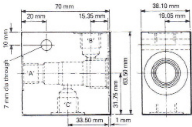
C200 Valve block HSP1619 3 ports 3/8" BSPF
