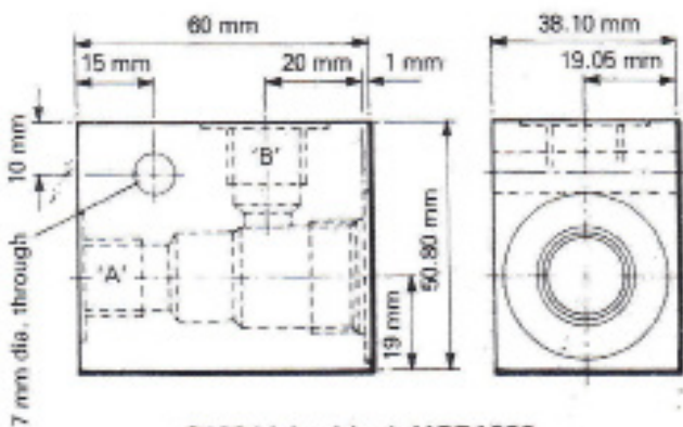
C100 Valve block HSP1620 2 ports 3/8" BSPF
