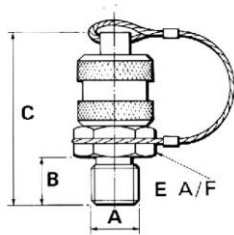
BSPP Plug Assembly
