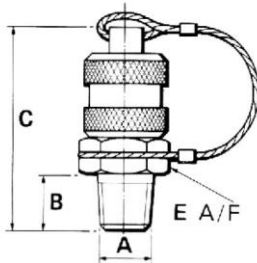
NPTF & BSPT Plug Assembly
