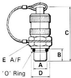
SAE & JIS.B.2401 Plug Assembly
