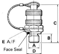
Metric Plug Assembly (with metric/BSPP threads)
